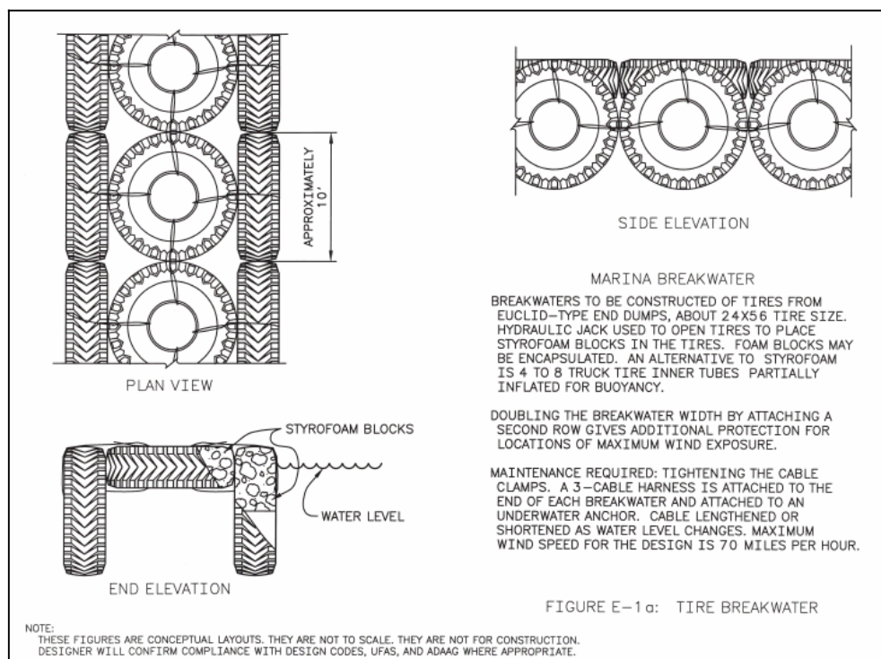
Fig. 36. Tire structure breakwater design from the Bureau of Reclamation ( http://www.usbr.gov/pmts/architecture/recfac/RFG-ch3.pdf ).
